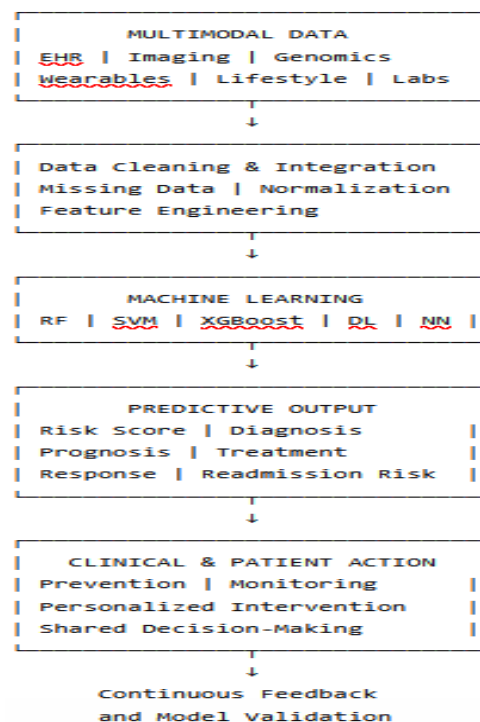
Figure 1. Conceptual framework for ML-enabled predictive healthcare
